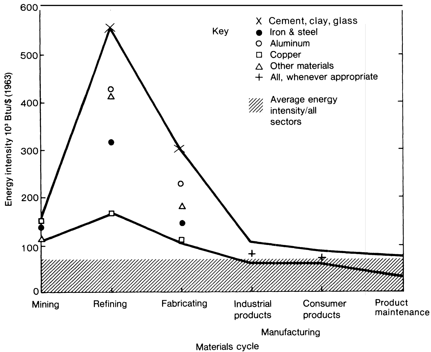
Figure 30.—Energy intensity at Each Stage of the Materials Cycle
