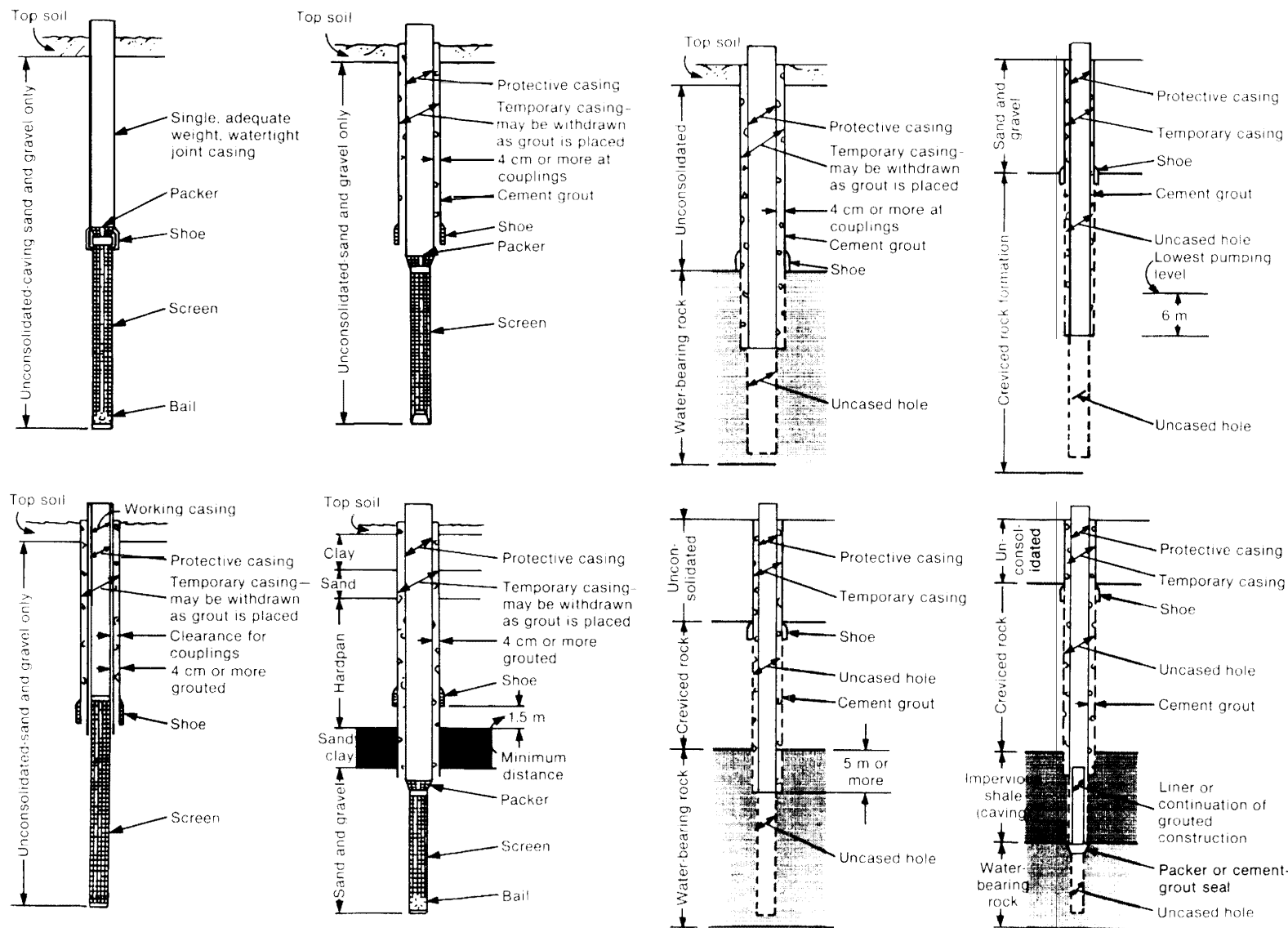
Figure 67.—Examples of Different Types of Wells
