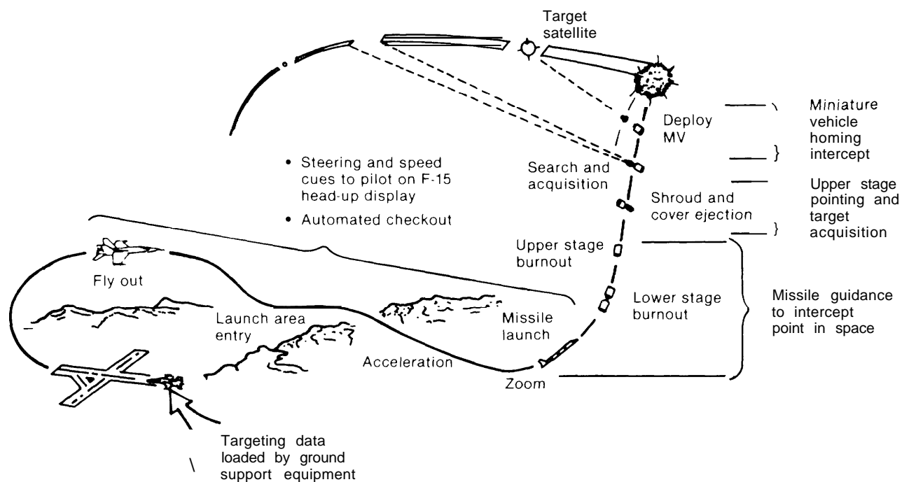
Figure 4-10. —ASAT Mission Profile
