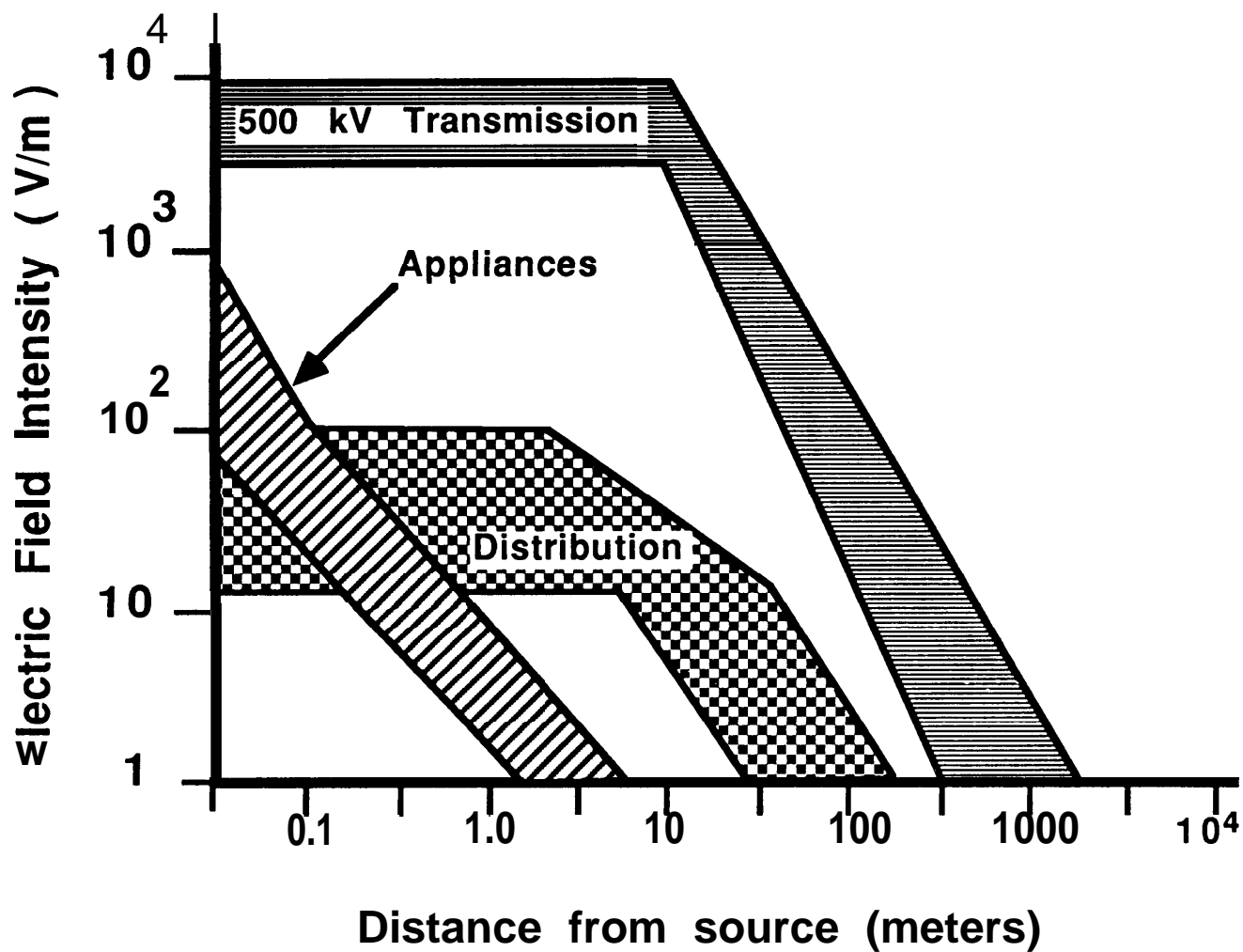
Figure 2-5: Illustration of how the electric field intensity at ground level changes with horizontal distance from three common sources of power-frequency electric fields. The bands represent variation across individual sources in each group. Adapted from [Florig 87a].
