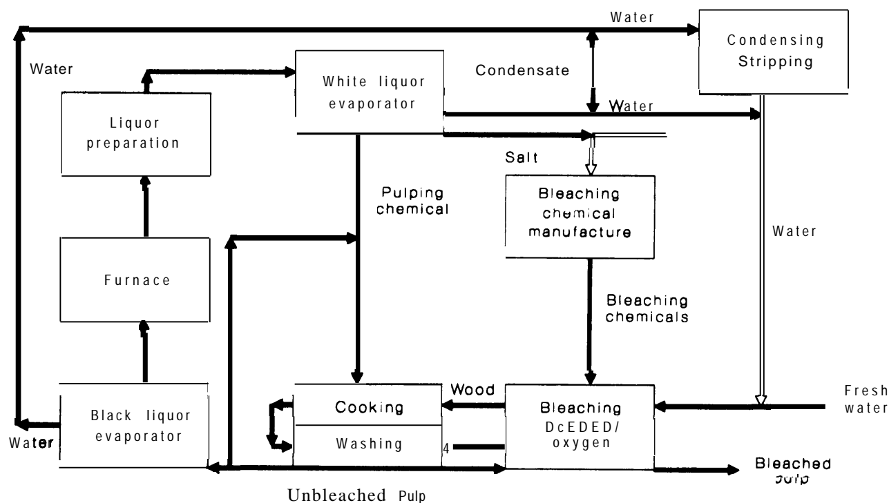
Figure 5-8—Closed-Cycle Bleached Kraft Pulp Mill
