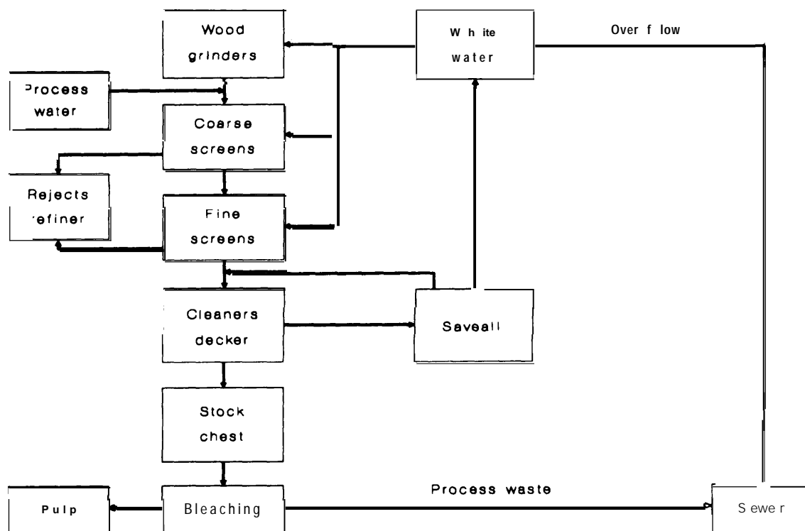
Figure 2-2-Stone Groundwood Pulp Mill Flow
