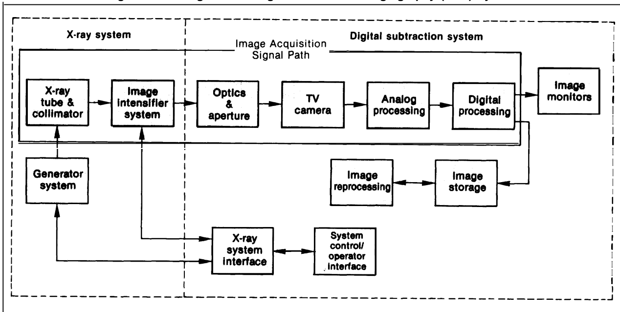
Figure 3-1.—Diagram of a Digital Subtraction Angiography (DSA) System
