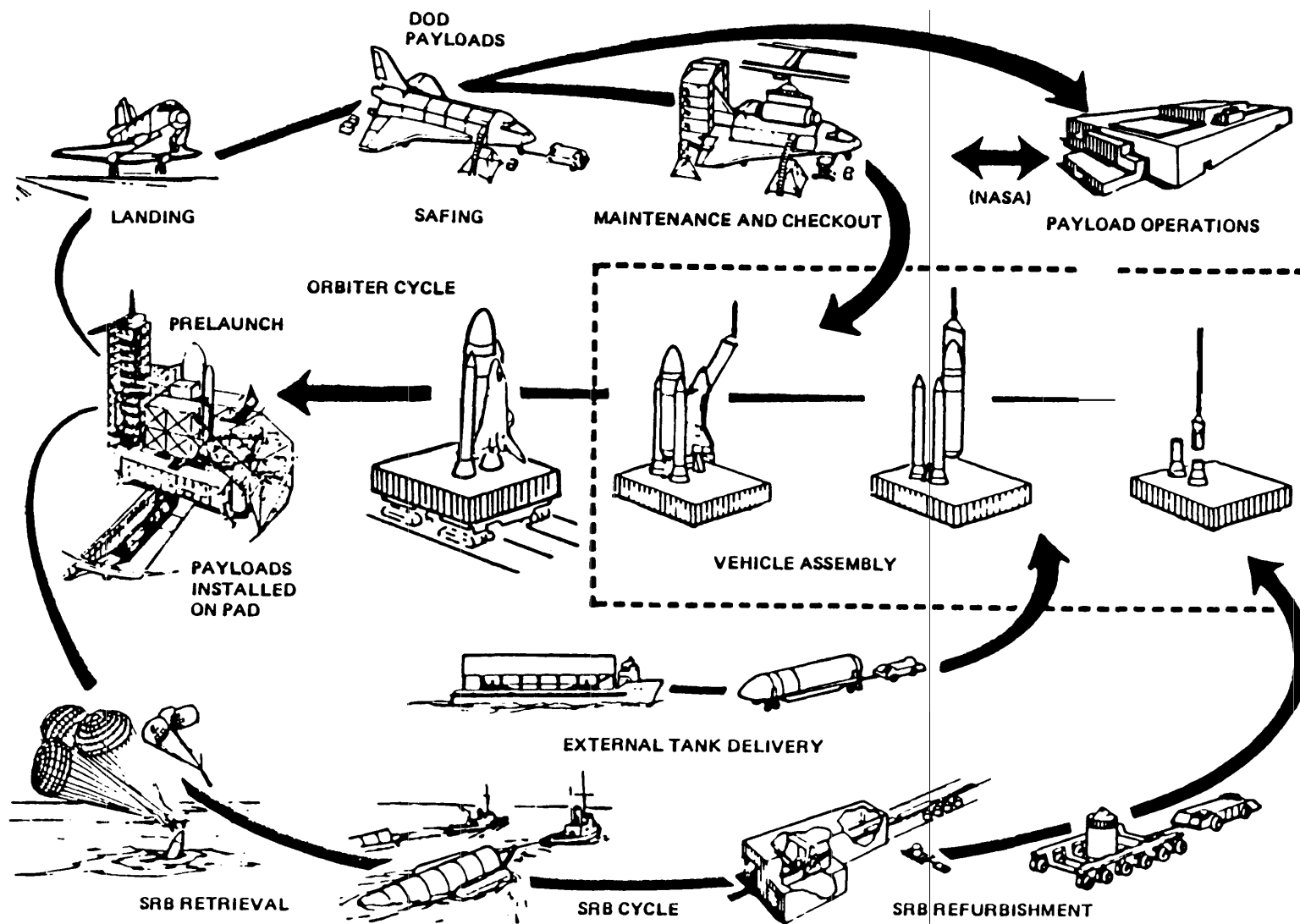
Figure 3-3—Kennedy Space Center Space Shuttle System Ground Flow
