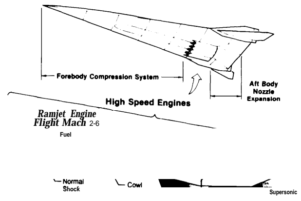
Figure 5-4-High-Speed Propulsion System
