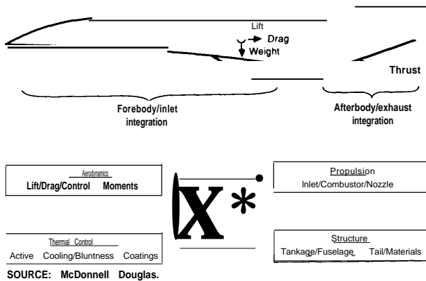
Figure 5-1--System Integration
