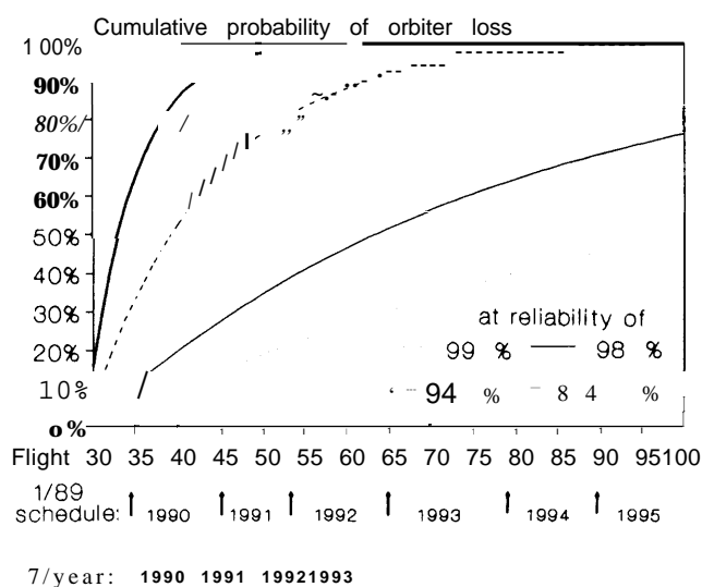
Figure 3-5-Effect of Flight Rate on Shuttle Orbiter Attrition
