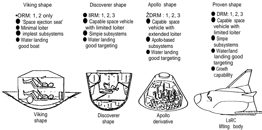
Figure 6-2--Design Reference Missions (DRMs)
