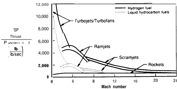
Figure 5-5—Engine I_{sp}
