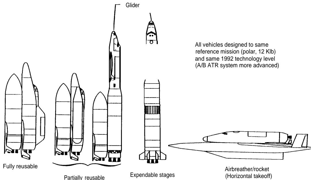
Figure 4-1-Advanced Manned Launch System Concepts
