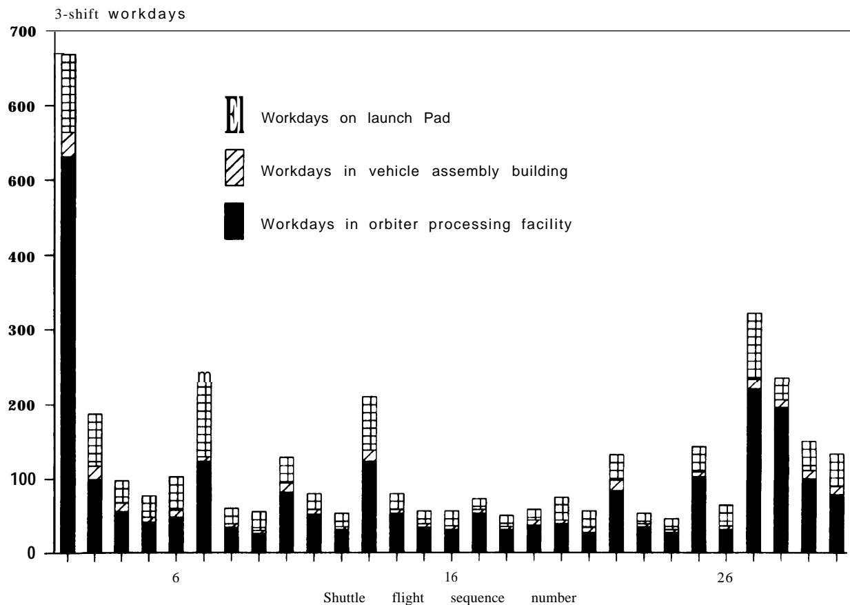
Figure 34-Orbiter Ground Turnaround Experience
