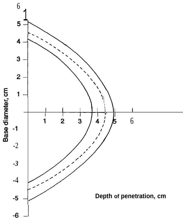
Figure A-2—The .38-Caliber Deformation Envelope in 20 Percent Ballistic Gelatin Backing 7-Ply, 400/2-Denier Kevlar 29 Armor Struck by 158-Grain, .38-Caliber Bullets
